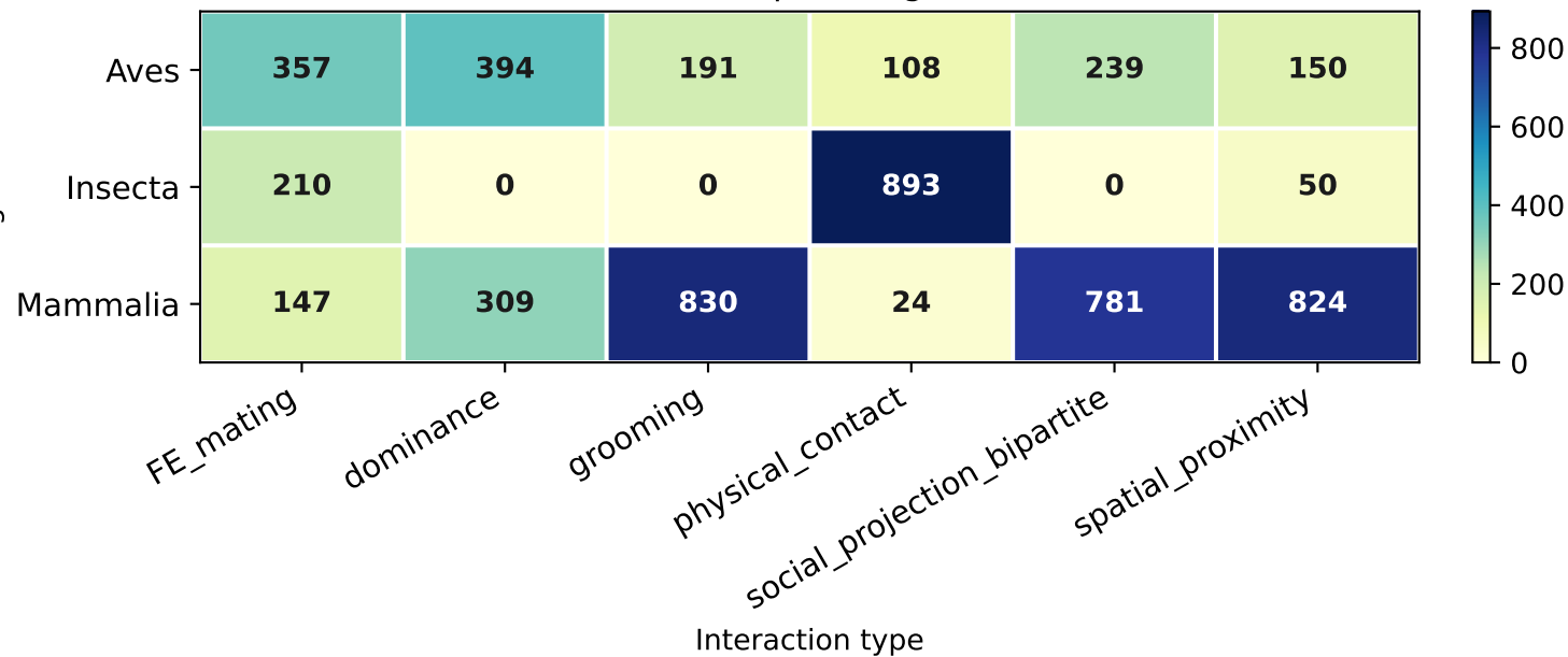
Raw counts — post-augmentation
